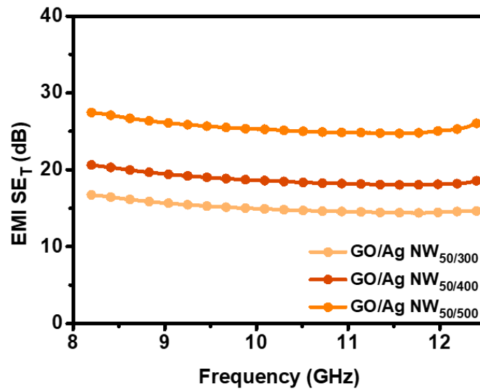
Fig. S5 EMI SE T value of the GO/Ag NW films
