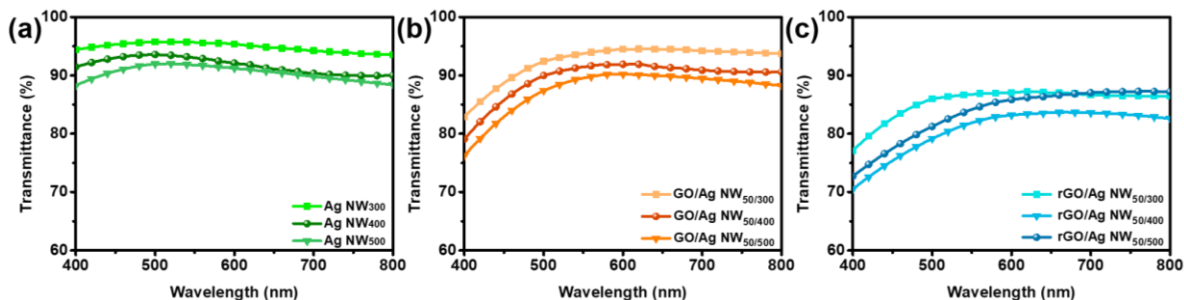
Fig. S3 Optical transmittance of a Ag NW, b GO/Ag NW, c rGO/Ag NW
