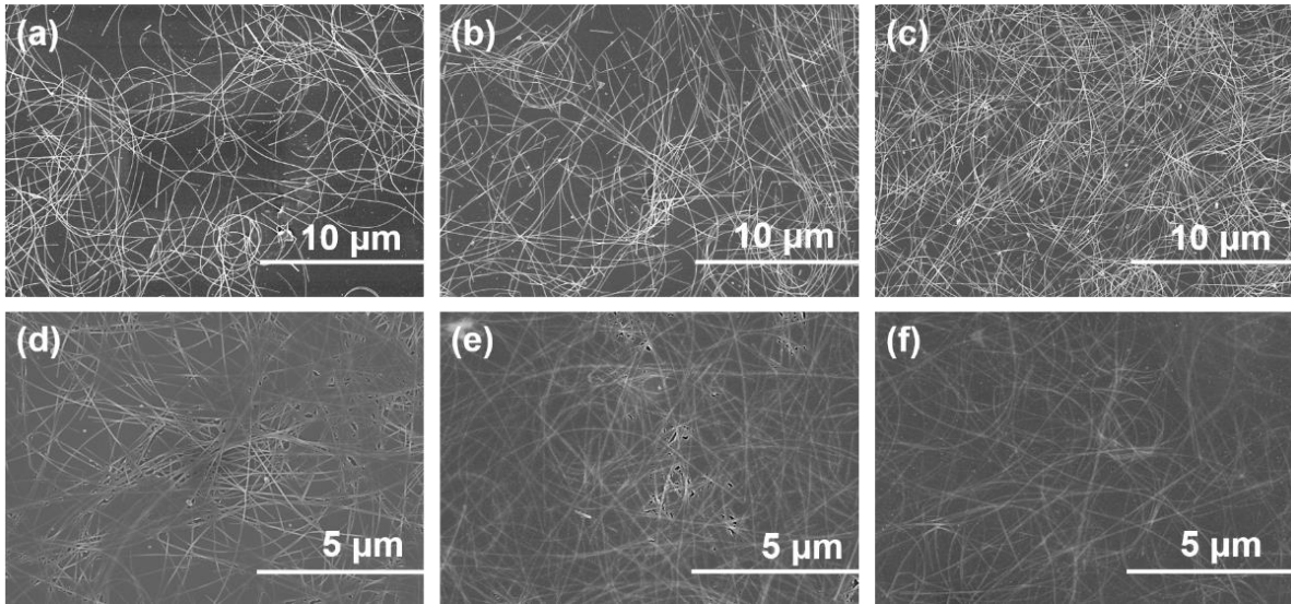
Fig. S4 SEM images a Ag NW 300 , b Ag NW 400 , c Ag NW 500 . SEM images of the rGO/Ag NW film with various rGO area density of d 30 mg·m -2 , e 40 mg·m -2 , f 50 mg·m -2
