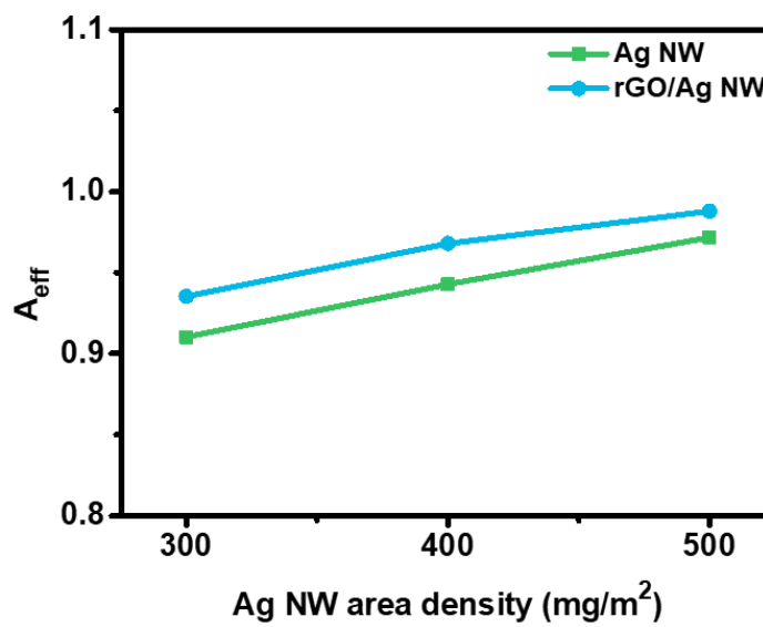
Fig. S6 A eff of the Ag NW and rGO/Ag NW films
