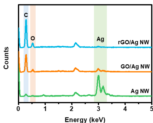
Fig. S1 The EDS spectra of the Ag NW, GO/Ag NW, and rGO/Ag NW films
