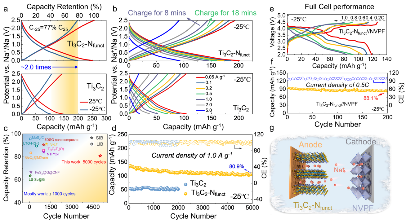
Fig. 3 Electrochemical performance of \text{Ti}_3\text{C}_2 and \text{Ti}_3\text{C}_2\text{-N}_{\text{funct}} anodes in Na-ion half-cells and \text{Ti}_3\text{C}_2\text{-N}_{\text{funct}} //NVPF full-cell. a The second charge/discharge curves of \text{Ti}_3\text{C}_2 and \text{Ti}_3\text{C}_2\text{-N}_{\text{funct}} anodes in Na-ion half-cells at 0.05 \text{A g}^{-1} under 25 and -25\text{ }^\circ\text{C} . b Rate capabilities of half-cells at -25\text{ }^\circ\text{C} . c Comparison of low-T cycle performance of \text{Ti}_3\text{C}_2\text{-N}_{\text{funct}} vs. other reported LIBs and SIBs. d Cycle performance of half cell at -25\text{ }^\circ\text{C} . e Rate performance (1C represents 0.128 \text{mA g}^{-1} ) and f cycling stability at 0.5C of \text{Ti}_3\text{C}_2\text{-N}_{\text{funct}} //NVPF full-cell. g Illustration of \text{Ti}_3\text{C}_2\text{-N}_{\text{funct}} //NVPF full-cell
