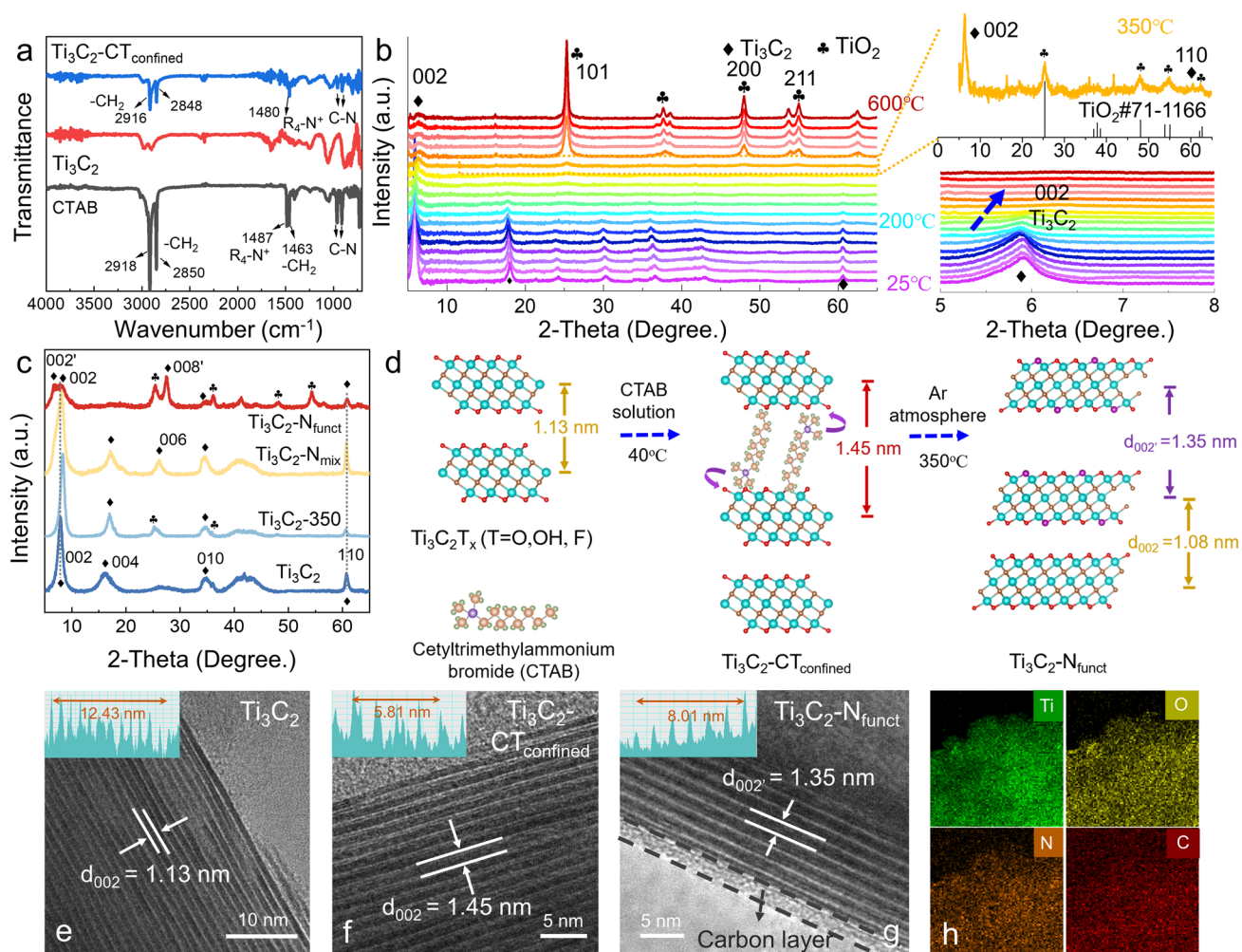
Fig. 1 a FTIR spectra of CTAB powder, \text{Ti}_3\text{C}_2 and \text{Ti}_3\text{C}_2\text{-CT}_{\text{confined}} . b In situ high-temperature XRD patterns, enlarged view within 5^\circ\text{--}8^\circ of \text{Ti}_3\text{C}_2\text{-CT}_{\text{confined}} within 25\text{--}600^\circ\text{C} , and enlarged view of XRD pattern at 350^\circ\text{C} . c XRD patterns of \text{Ti}_3\text{C}_2 , \text{Ti}_3\text{C}_2\text{-350} , \text{Ti}_3\text{C}_2\text{-N}_{\text{mix}} and \text{Ti}_3\text{C}_2\text{-N}_{\text{funct}} . d Illustration of \text{Ti}_3\text{C}_2 during the tailoring process. HRTEM images of e \text{Ti}_3\text{C}_2 , f \text{Ti}_3\text{C}_2\text{-CT}_{\text{confined}} and g \text{Ti}_3\text{C}_2\text{-N}_{\text{funct}} . h Ti, O, N, and C elements mappings of \text{Ti}_3\text{C}_2\text{-N}_{\text{funct}}
