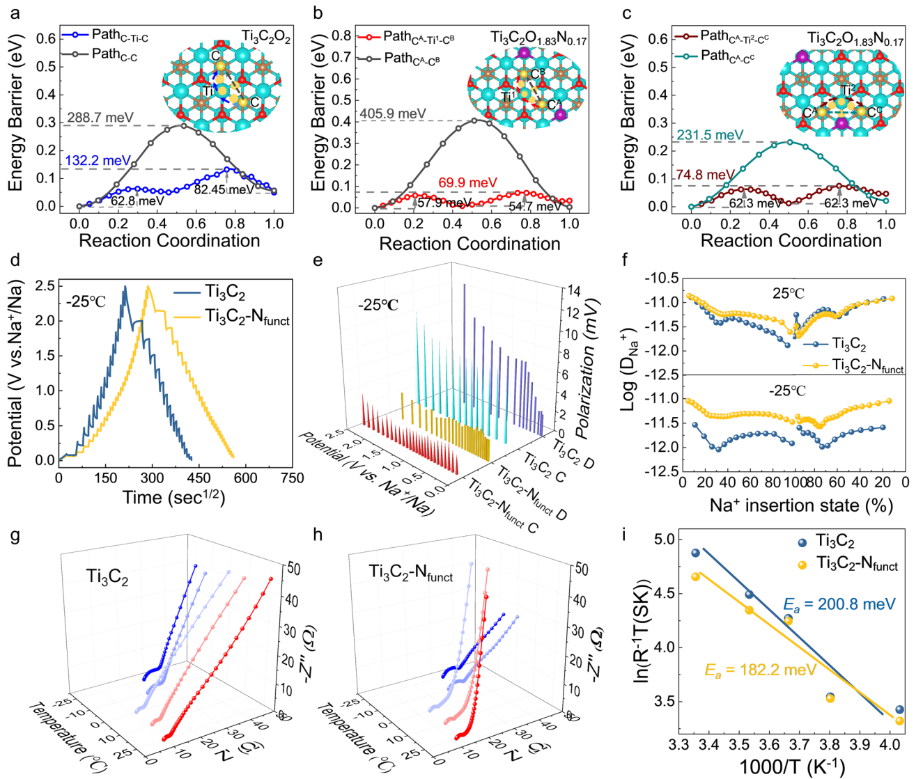
Fig. 4 Kinetics analysis: the diffusion energy barrier of Na + along different paths in a Ti 3 C 2 O 2 and b-c Ti 3 C 2 O 1.83 N 0.17 . d Charge–discharge GITT curves of Ti 3 C 2 and Ti 3 C 2 -N funct . e Comparison of polarization of the two electrodes at -25 °C during the charge/discharge process. f The Na + diffusion coefficients of Ti 3 C 2 and Ti 3 C 2 -N funct at 25 °C and -25 °C. Temperature-dependent EIS study of g Ti 3 C 2 and h Ti 3 C 2 -N funct anodes from -25 to 25 °C. i Arrhenius plot of the resistance contributions of the charge transfer resistance ( R ct ) with the derived activation energies ( E a ) for the two electrodes
