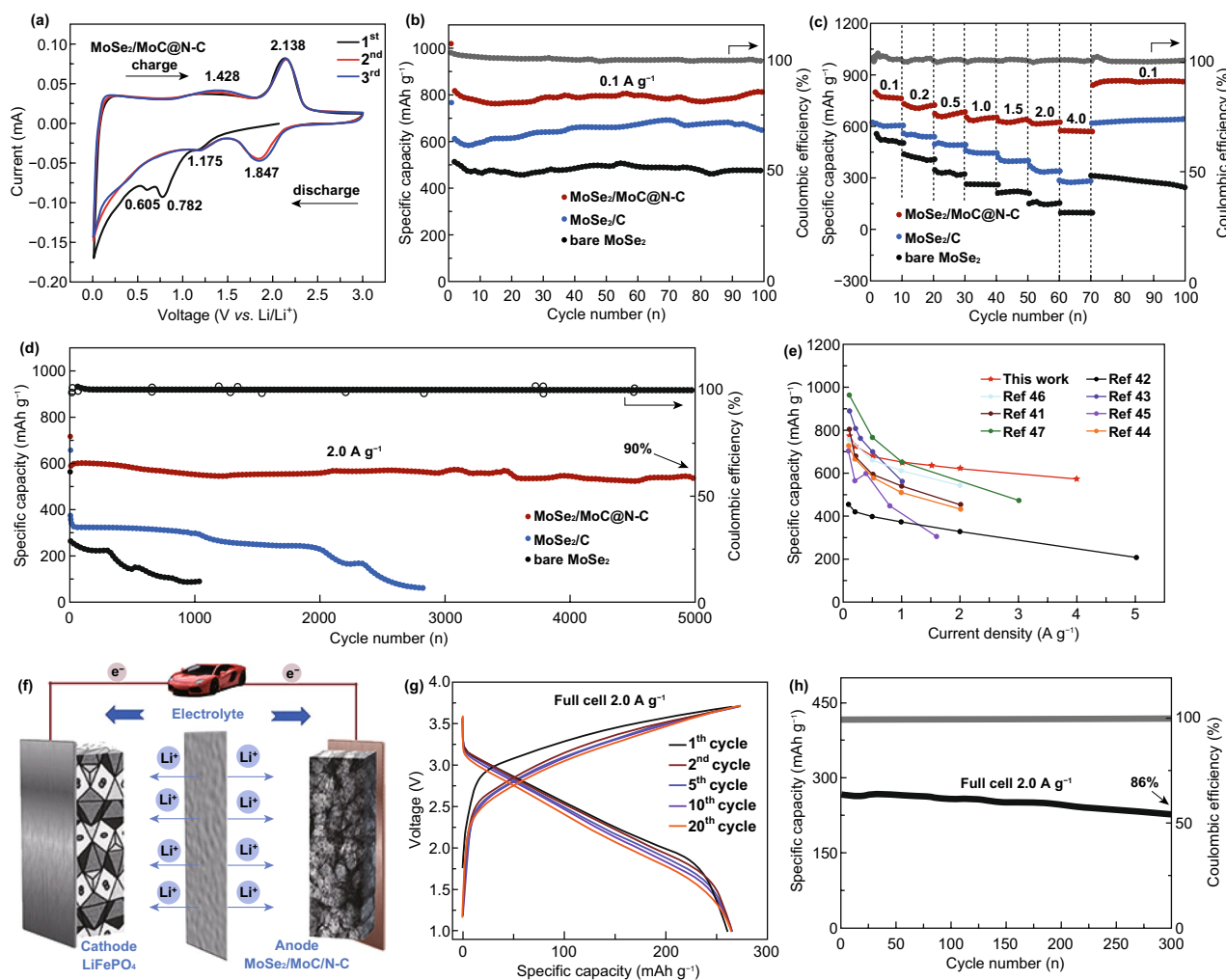
Fig. 3 a Initial three cyclic voltammograms cycles of the \text{MoSe}_2/\text{MoC}/\text{N-C} electrode at a scan rate of 0.1 \text{ mV s}^{-1} . b Cycling performance ( 0.1 \text{ A g}^{-1} ), c rate performances, and d long-term cycling performances ( 2 \text{ A g}^{-1} ) of bare \text{MoSe}_2 , \text{MoSe}_2/\text{C} , and \text{MoSe}_2/\text{MoC}/\text{N-C} electrodes between 0.01 and 3 V versus \text{Li}/\text{Li}^+ . e Comparison plot of rate performance between this work and previously published \text{MoSe}_2/\text{C} composite-related works. f Schematic illustration of the \text{LiFePO}_4/\text{MoSe}_2/\text{MoC}/\text{N-C} full-cell configuration. g Charge/discharge profiles of the full cell. h Cycling performance of the full cell at 0.1 \text{ A g}^{-1}
