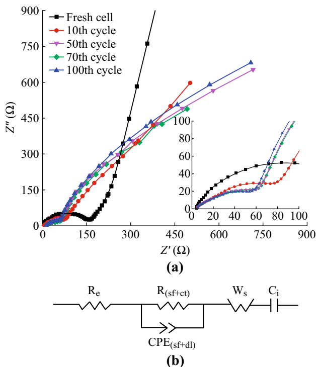
Fig. 9 a Electrochemical impedance spectra of ZnCo 2 O 4 NCPs electrode after different cycles. b Equivalent electrical circuit used to fit the data of Fig. 9a
