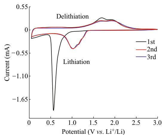
Fig. 7 Cyclic Voltammograms of \text{ZnCo}_2\text{O}_4 NCPs electrode at a scan rate of 0.1 \text{ mV s}^{-1}
