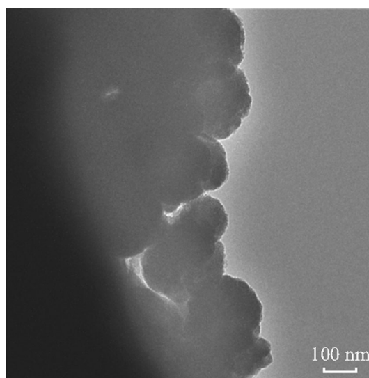
Fig. 8 TEM image of \text{ZnCo}_2\text{O}_4 NCPs electrode after 100 cycles at 100 \text{ mA g}^{-1}
