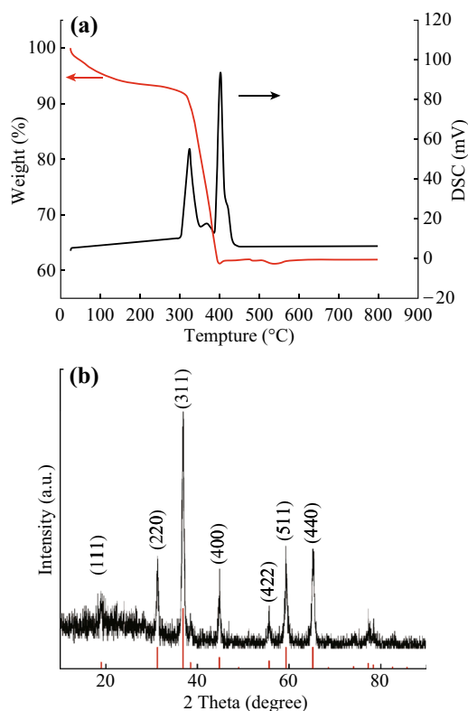
Fig. 1 a TG–DTA of the precursor; b XRD of ZnCo 2 O 4 NCPs
