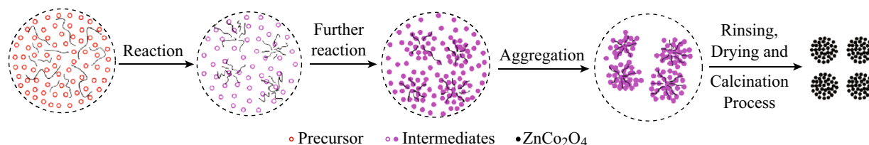
Scheme 1 Illustration of the formation process of ZnCo 2 O 4 NCPs
