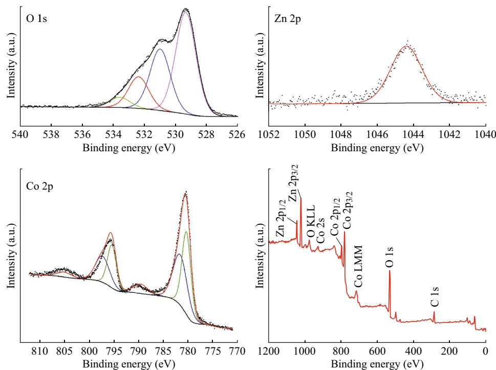
Fig. 2 XPS spectra: O 1s, Zn 2p, Co 2p, and survey spectrum for the as-synthesized \text{ZnCo}_2\text{O}_4 NCPs
