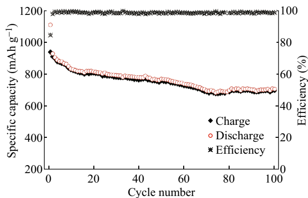
Fig. 5 Cycling performance at 0.1 °C for ZnCo 2 O 4 NCPs
