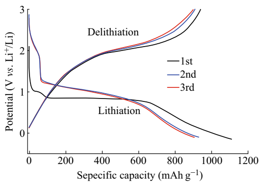
Fig. 4 The first three lithiation/delithiation curves of ZnCo 2 O 4 NCPs
