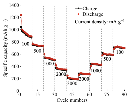
Fig. 6 Rate performance of \text{ZnCo}_2\text{O}_4 NCPs electrode at various current densities
