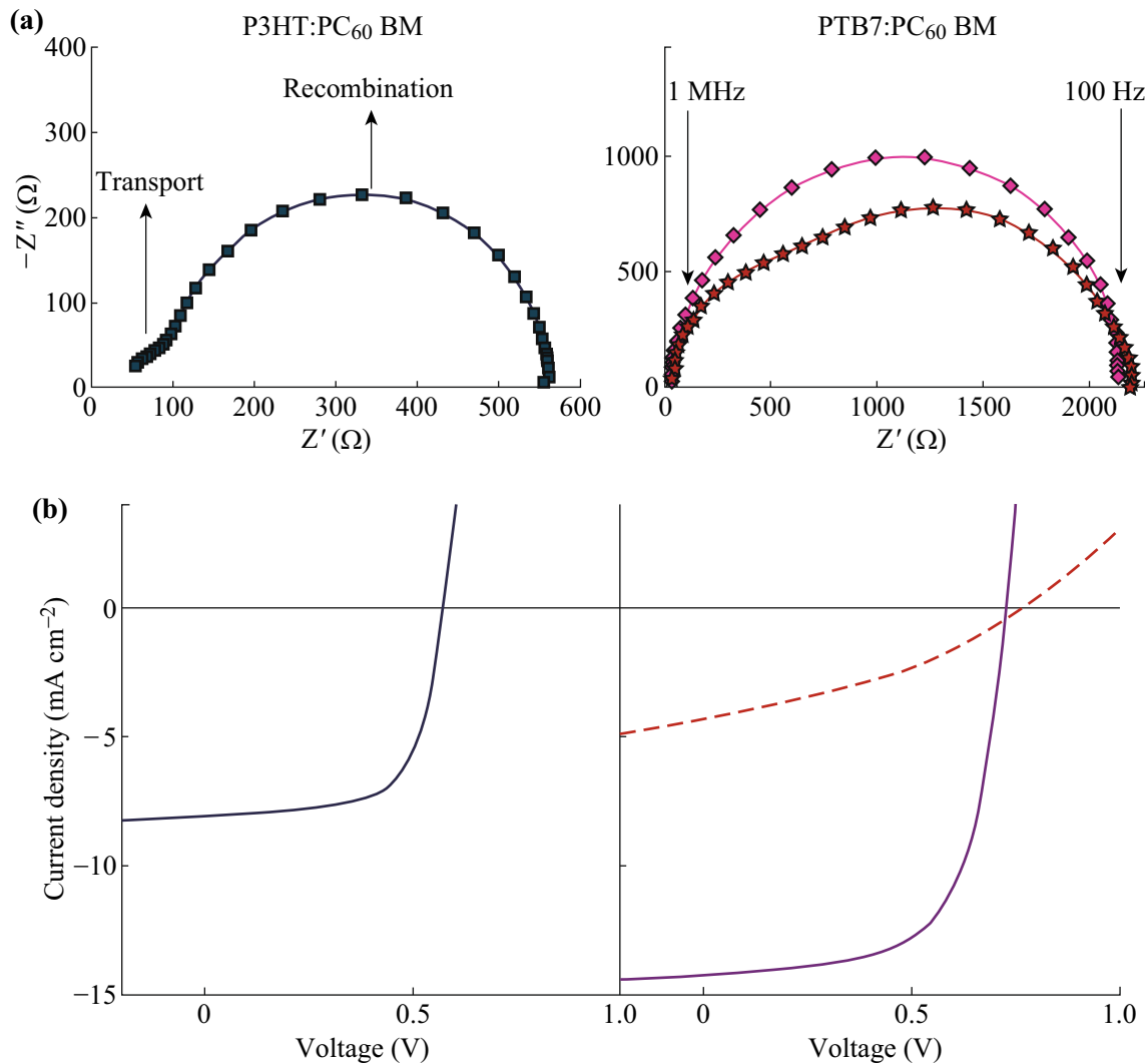
Fig. 2 Representative P3HT:PC60BM, PTB7:PC60BM devices that illustrate the differences in the observed IS response for devices measured at 1 sun light intensity, at applied voltages close to V_{oc} . Figure adapted with permission of Ref. [35]
