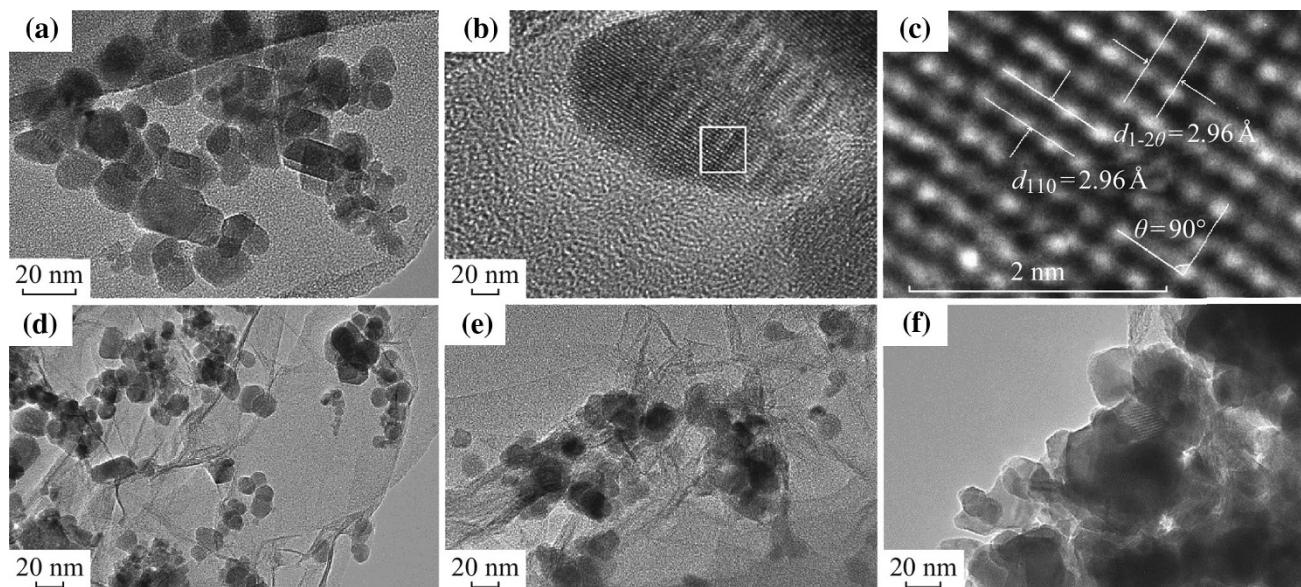
Fig. 2 TEM images of bare \text{CoFe}_2\text{O}_4 (a); \text{CoFe}_2\text{O}_4 -GNSs (d); \text{CoFe}_2\text{O}_4 -GNSs-350 (e); and \text{CoFe}_2\text{O}_4 -GNSs-550 (f). HRTEM images of \text{CoFe}_2\text{O}_4 (b, c)
