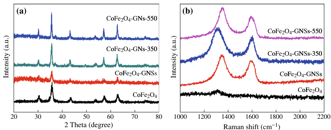
Fig. 1 XRD patterns (a) and Raman spectra (b) of \text{CoFe}_2\text{O}_4 , \text{CoFe}_2\text{O}_4\text{-GNSs} , \text{CoFe}_2\text{O}_4\text{-GNSs-350} , and \text{CoFe}_2\text{O}_4\text{-GNSs-550} , respectively
